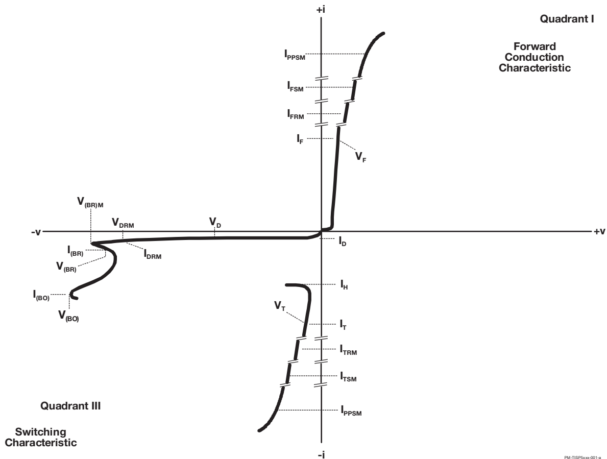
Figure 1. Voltage-Current Characteristic for Terminal Pair All All Measurements are Referenced to the Thyristor Anode, A (Pin 1)
